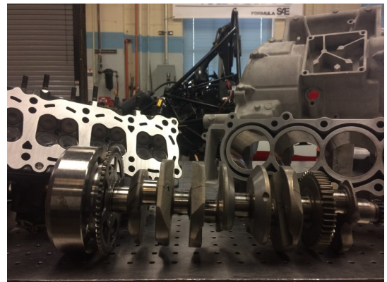
Right: Engine parts refinished by Hesco and US Chrome
